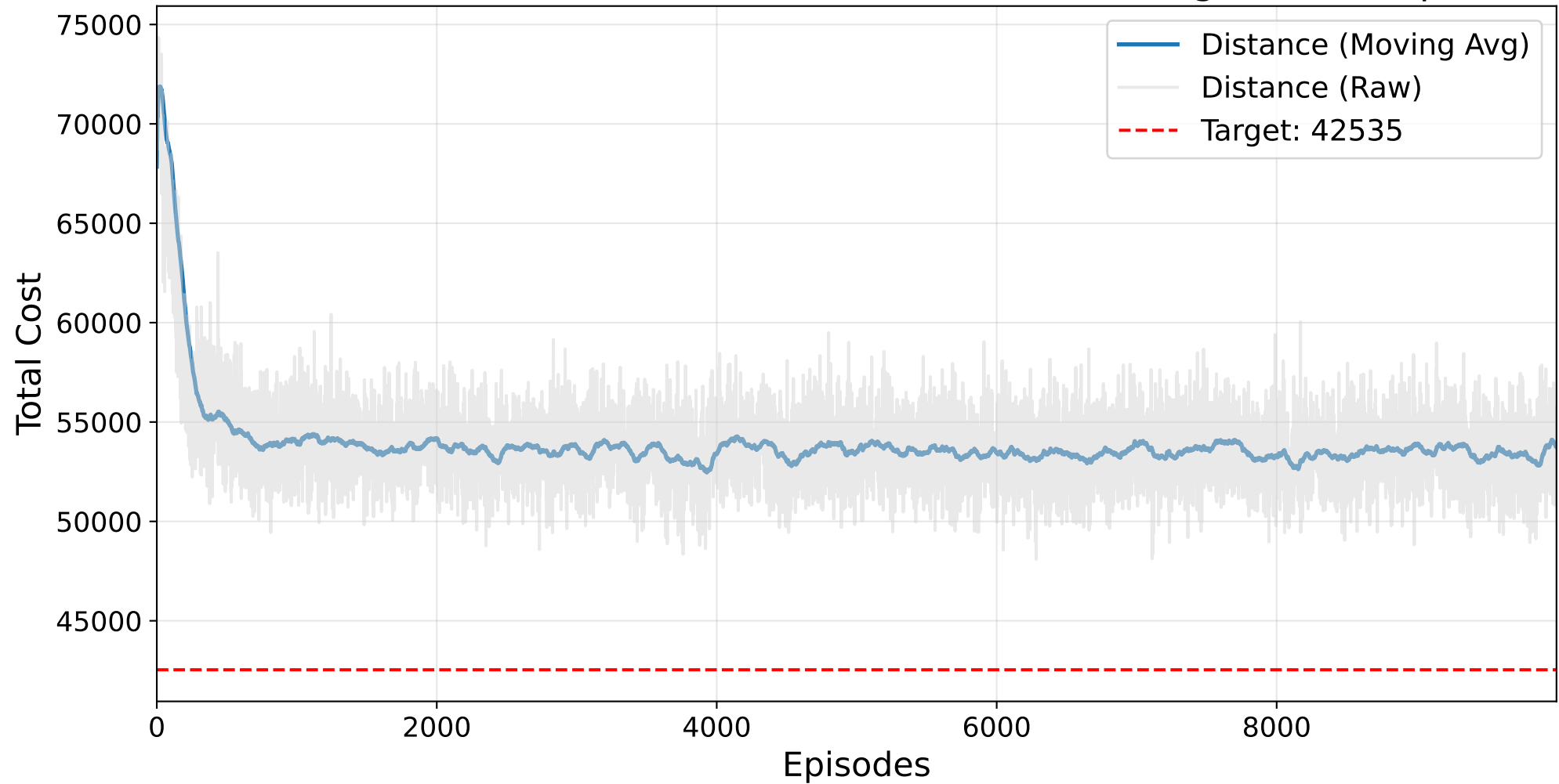
Final HYPERBAND GP Masked AutoRL-SOP Training - ft70.3.sop
